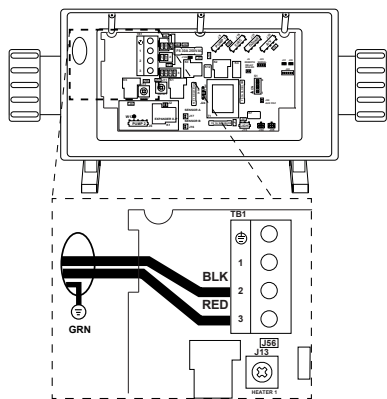
Figure C Connections (North American 60 Hz 240 VAC 3-Wire Connection Models)
