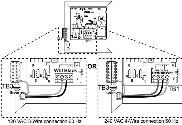
Figure D 120V/240V 60 Hz Convertible Models
